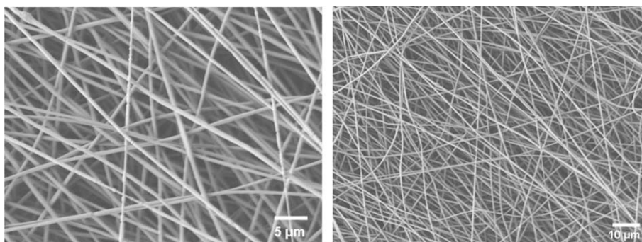
Fig. 2. SEM pictures of the electrospun silk mats. The mats consist of randomly distributed silk fibers of about 1 \mu m in diameter
